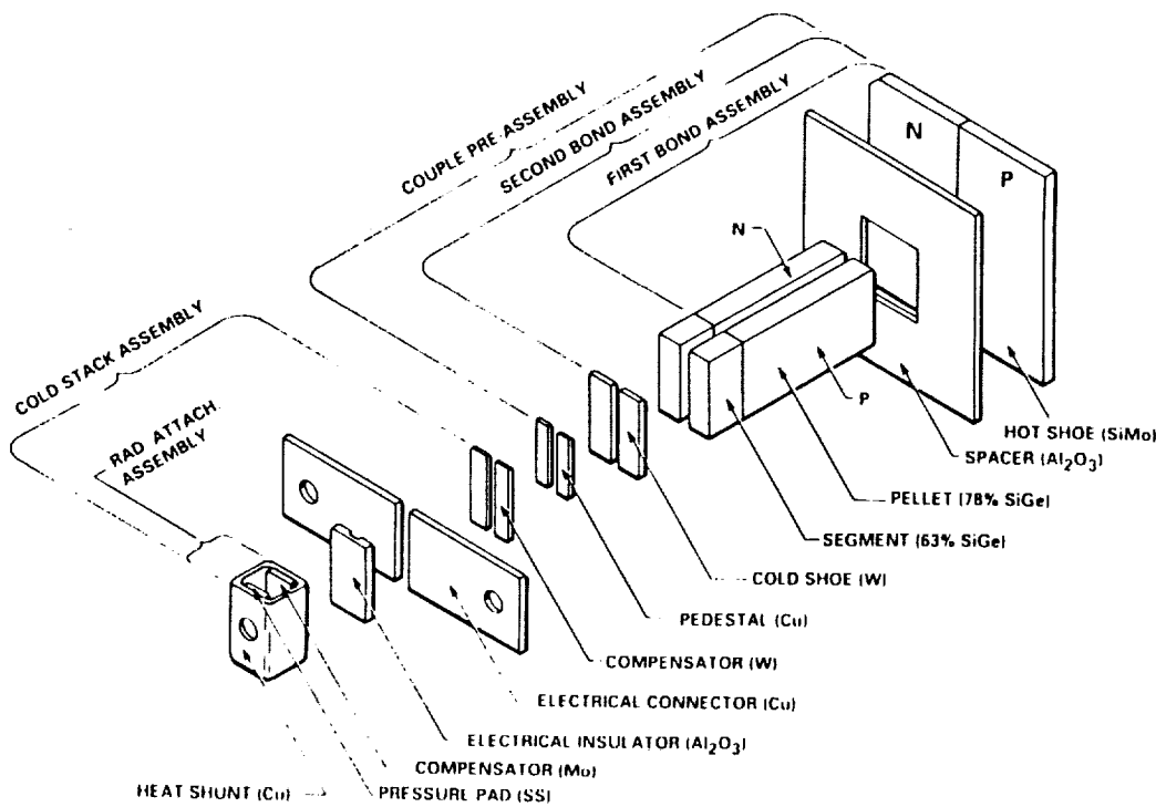
Figure 4. An exploded view of the silicon-germanium unicouple (thermoelectric element). 572 of these unicouples are used in each GPHS-RTG. The unicouple length is 3.11 centimeters and the hot shoe measures almost 2.3 centimeters by 2.3 centimeters. The hot shoe operating temperature is about 1305 K.
