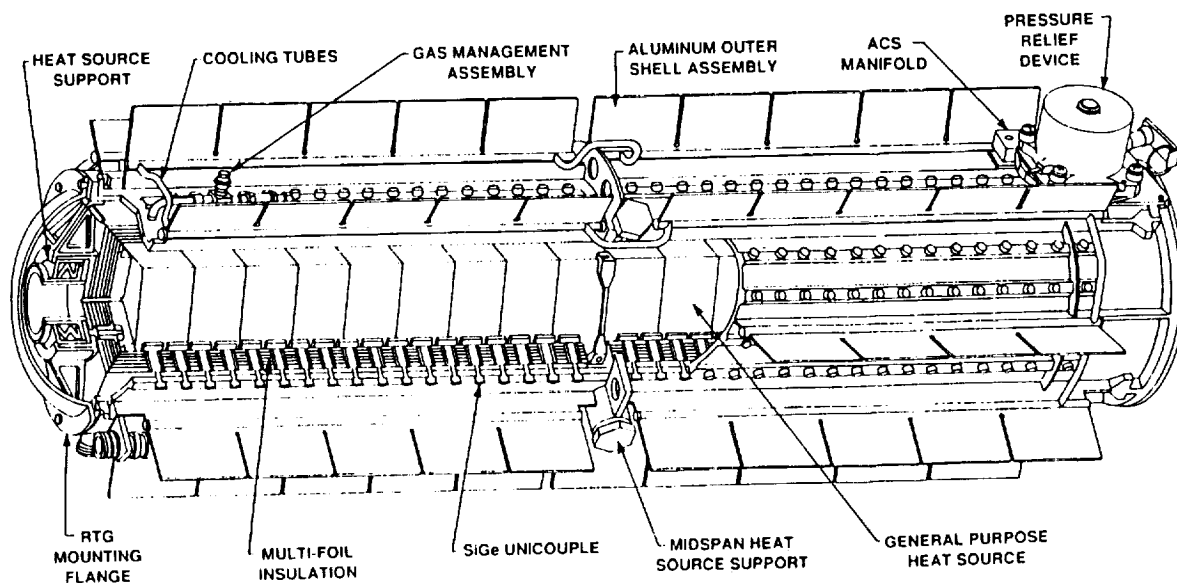
Figure 3. Cutaway drawing of the general-purpose heat source radioisotope thermoelectric generator (GPHS-RTG). The GPHS-RTG consists of two major components: the general purpose heat source (GPHS) and the converter which converts the thermal power generated in the GPHS into electrical power by means of 572 thermoelectric elements called "unicouples." The overall diameter of the GPHS-RTG with fins is 42.2 centimeters (about 16.6 inches). The mass of the GPHS-RTG is about 55.9 kilograms (weight of about 123 pounds). The GPHS-RTG produces over 300 watts of electrical power at the time of assembly. The GPHS-RTG has no moving parts and should provide power for over 20 years after launch.
