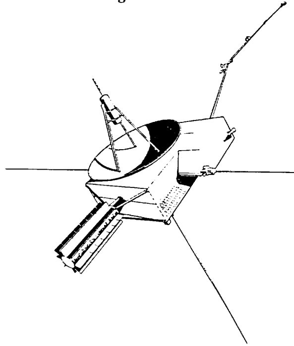
Figure 2. Diagram of the Ulysses spacecraft showing the general-purpose heat source radioisotope thermoelectric generator (GPHS-RTG) mounted on the side. Ulysses is a European Space Agency (ESA) spacecraft mission that was launched by NASA and has some U.S. experiments designed to study the polar regions of the Sun.
