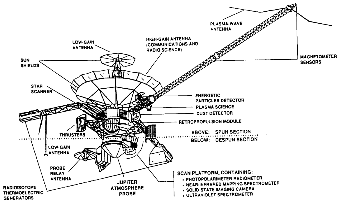
Figure 1. Diagram of the Galileo Orbiter and Probe showing the two general-purpose heat source radioisotope thermoelectric generators (GPHS-RTG) mounted on the two booms. The length of a GPHS-RTG is 113 centimeters (about 45 inches). Galileo is a NASA spacecraft mission to Jupiter, designed to study the planet's atmosphere, satellites and surrounding magnetosphere. Fully loaded with rocket fuel, the Orbiter has a mass of about 2400 kilograms (weight of about 5230 pounds). The Probe, which is designed to enter the atmosphere of Jupiter, has a mass of 340 kilograms (weight of about 750 pounds).
